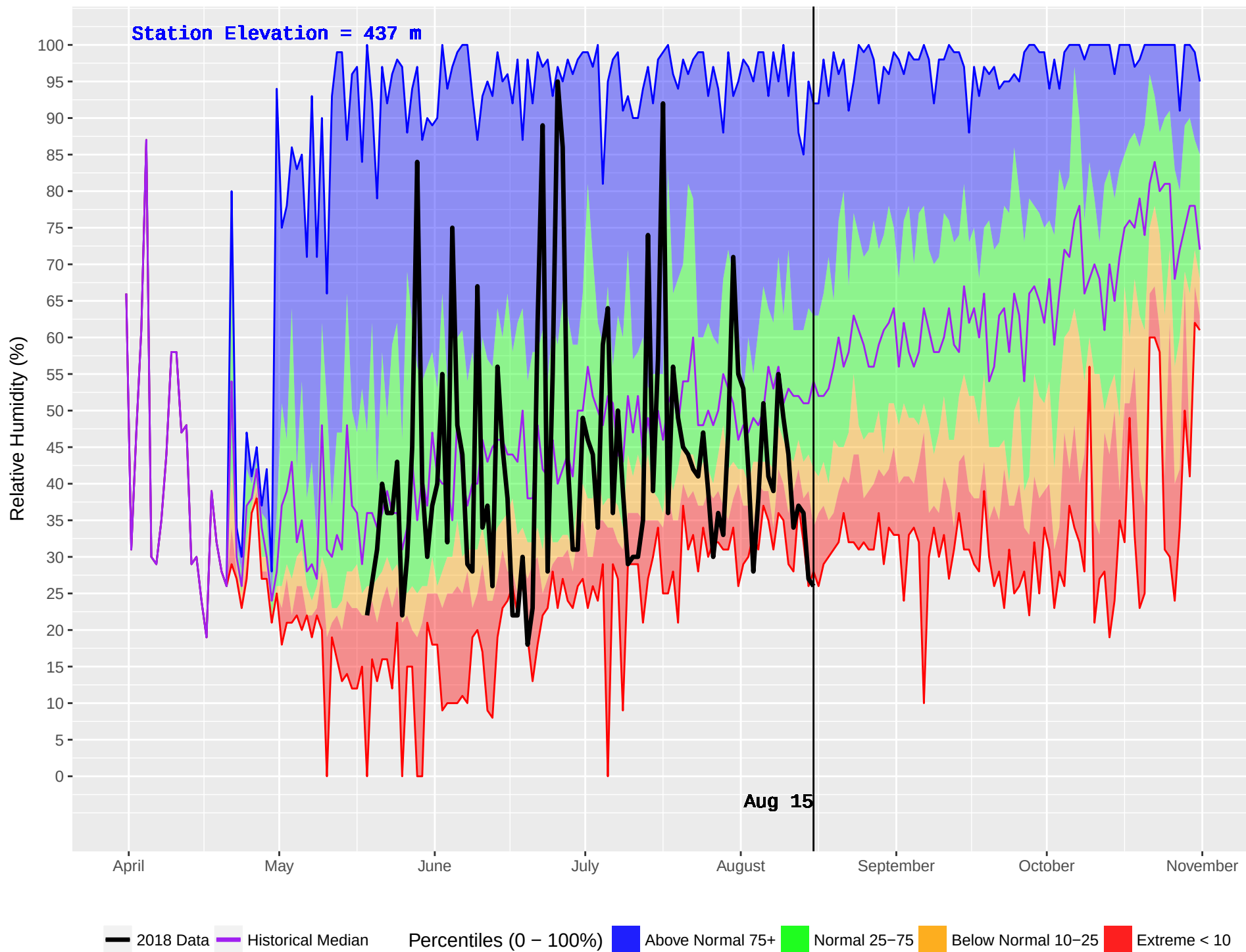
ELK MOUNTAIN (438) : Historical (1973–2016) and Current (2018) Daily Relative Humidity
