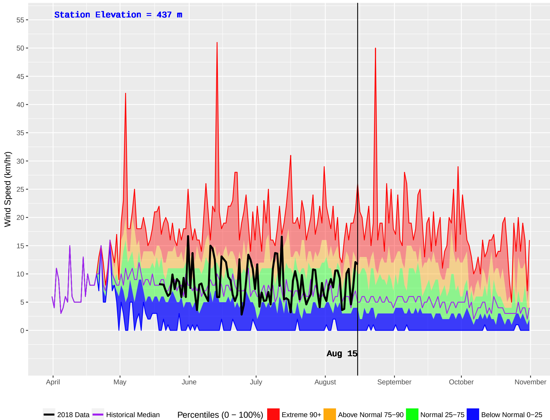
ELK MOUNTAIN (438) : Historical (1973–2016) and Current (2018) Daily Wind Speed
