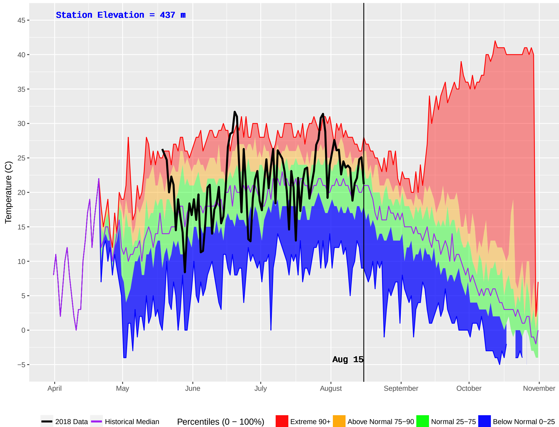
ELK MOUNTAIN (438) : Historical (1973–2016) and Current (2018) Daily Temperature
