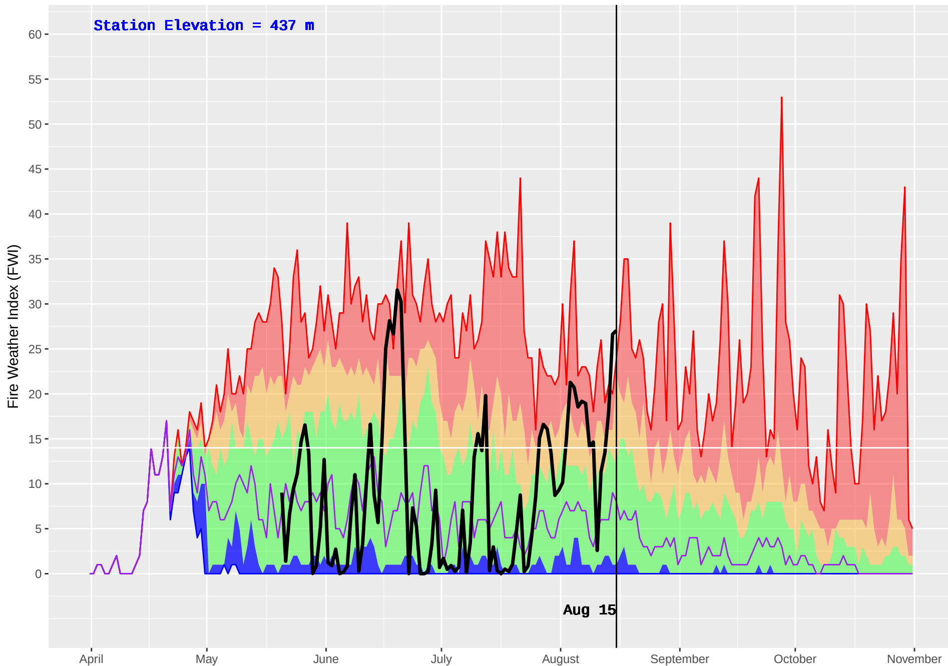
ELK MOUNTAIN (438) : Historical (1973–2016) and Current (2018) Daily Fire Weather Index (FWI)
